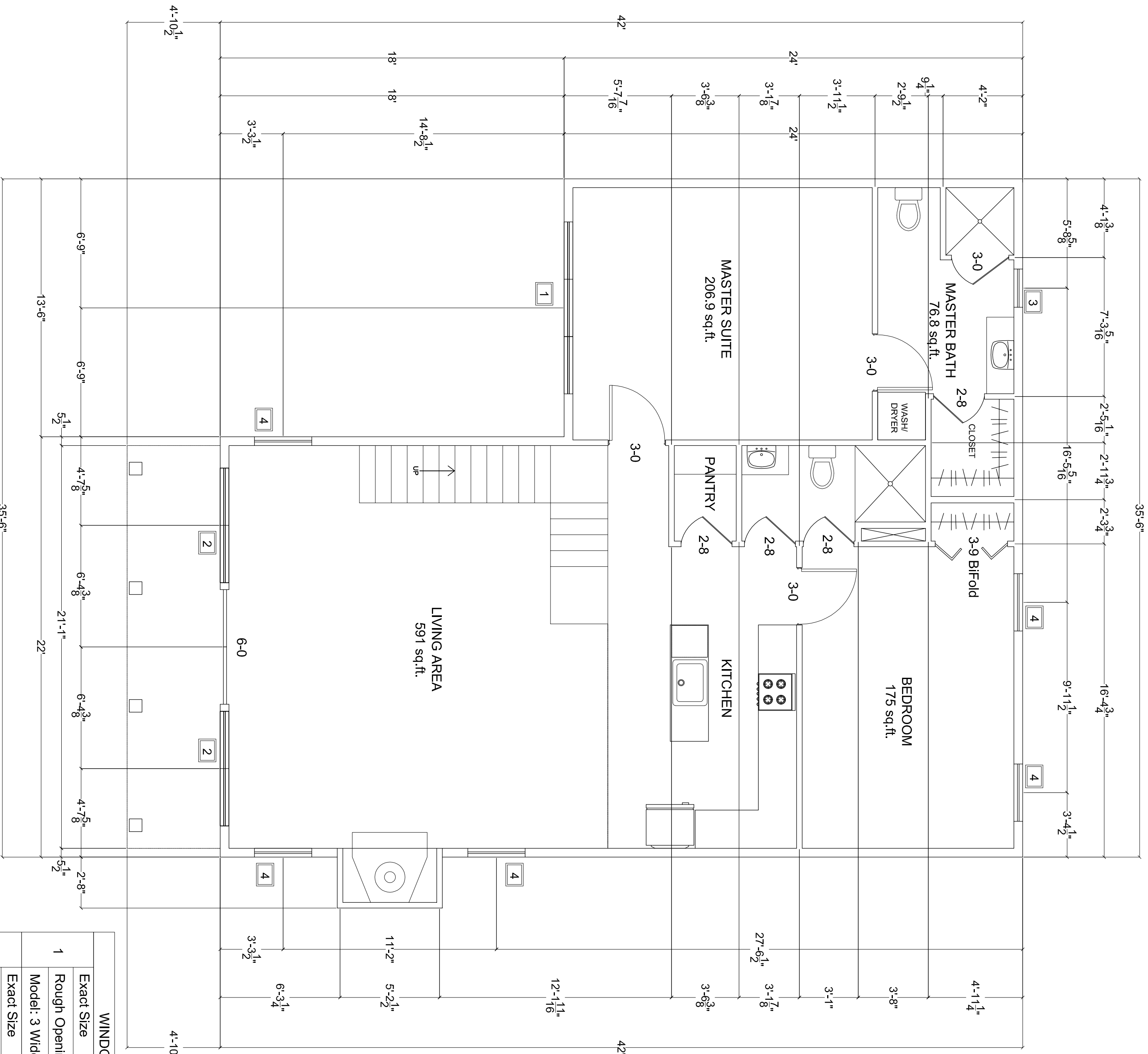
MAIN LEVEL 1,248 sq.ft.
