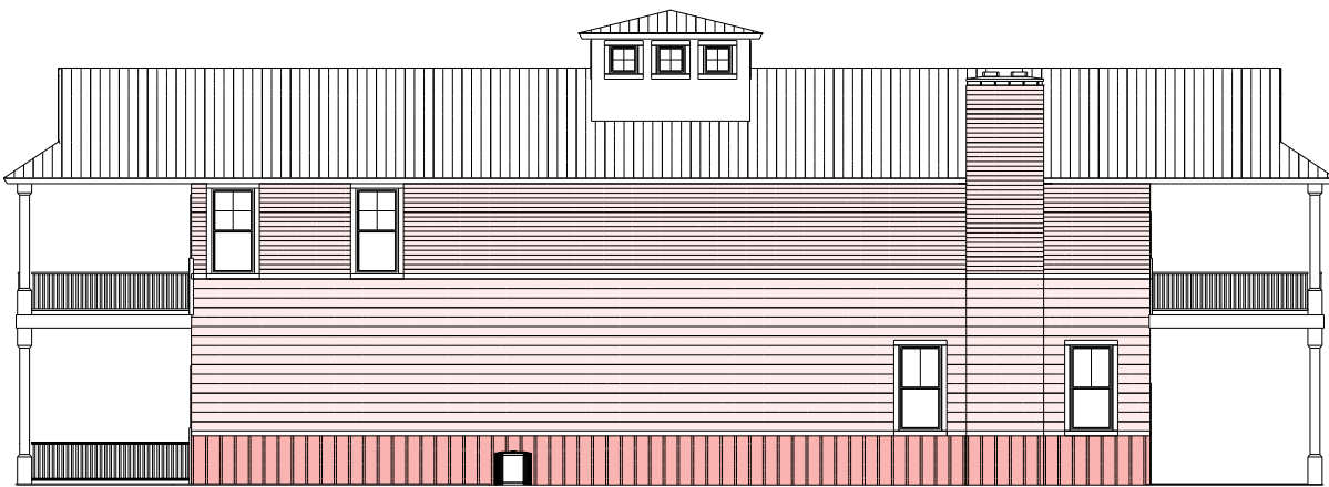
LEFT ELEVATION
